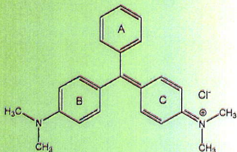
Chemical Structure
